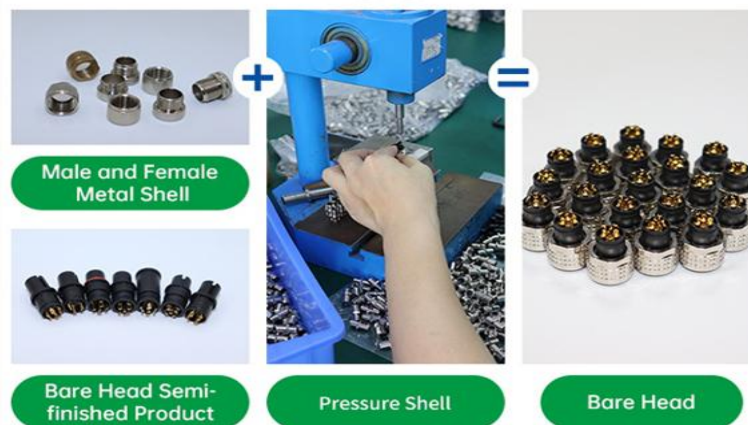
Bare Head Processing
